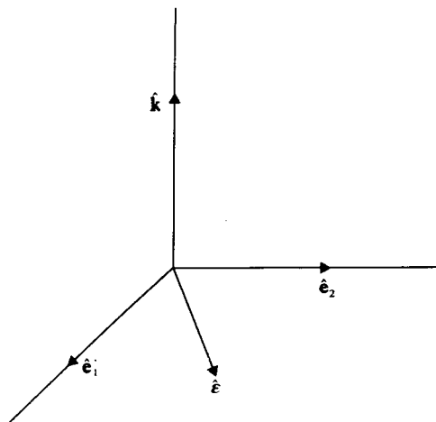
4.1 The vectors \hat{\mathbf{e}}_1 , \hat{\mathbf{e}}_2 and \hat{\mathbf{k}} , forming a right-handed set of mutually orthogonal unit vectors. Also shown is the polarisation vector \hat{\boldsymbol{\varepsilon}} which lies in the plane of \hat{\mathbf{e}}_1 and \hat{\mathbf{e}}_2 .
